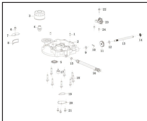
Crankcase cover
