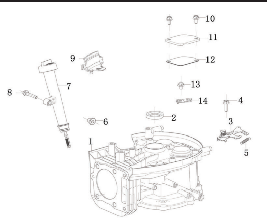
Crankcase body
