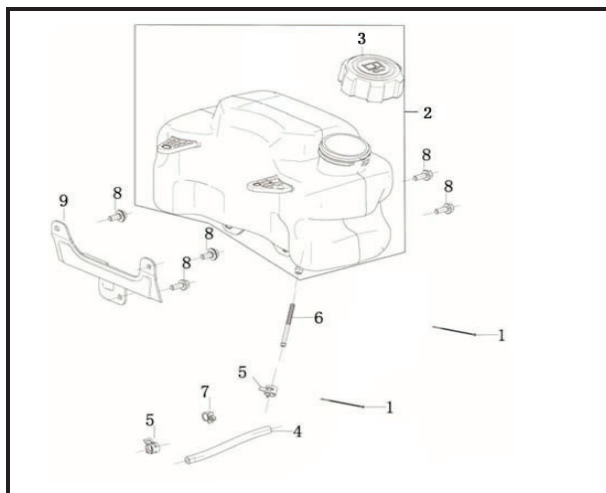
Fuel Tank
