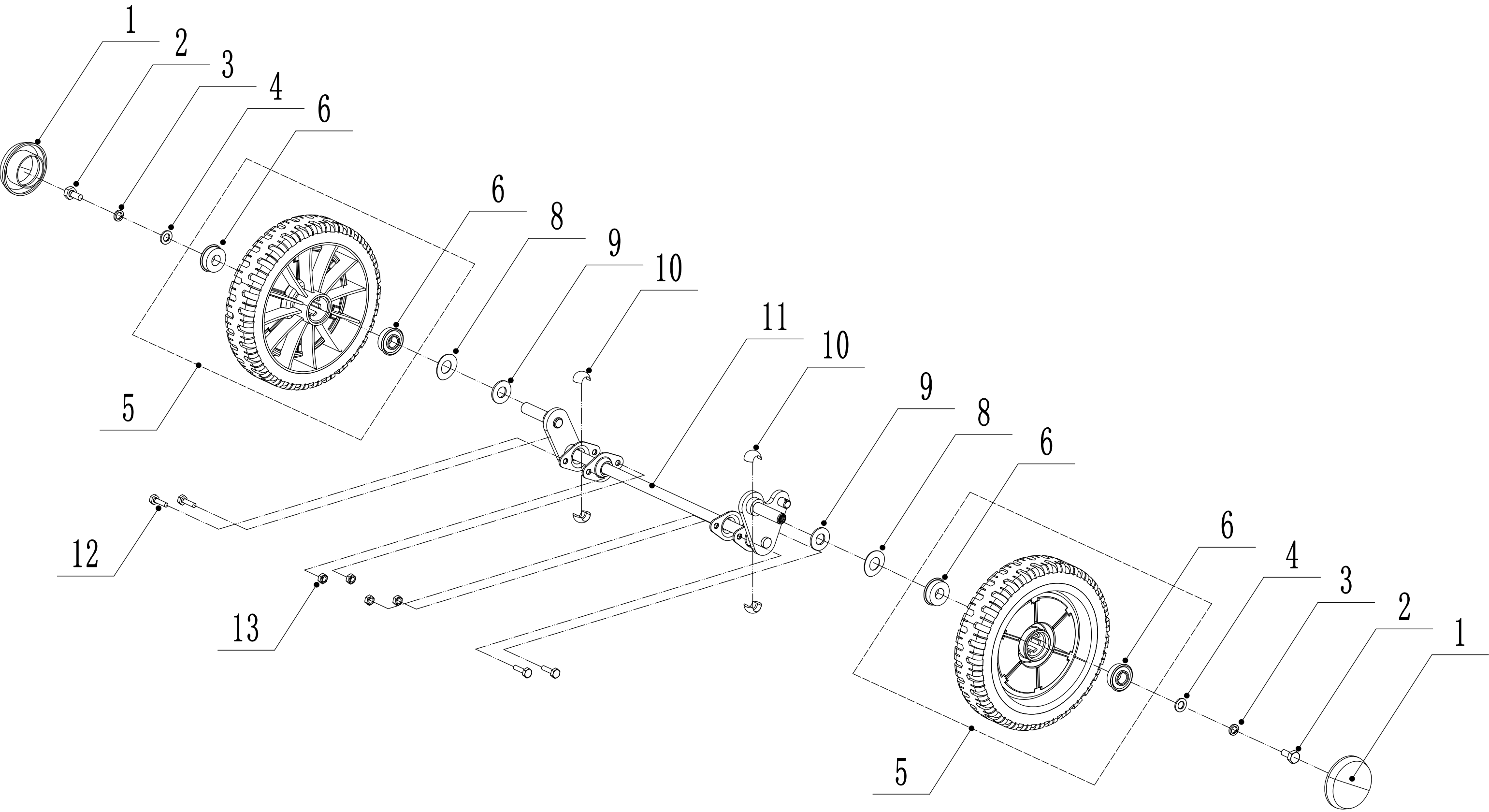
4 Front Axle
