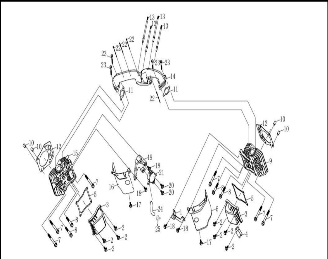
Cylinder Head
