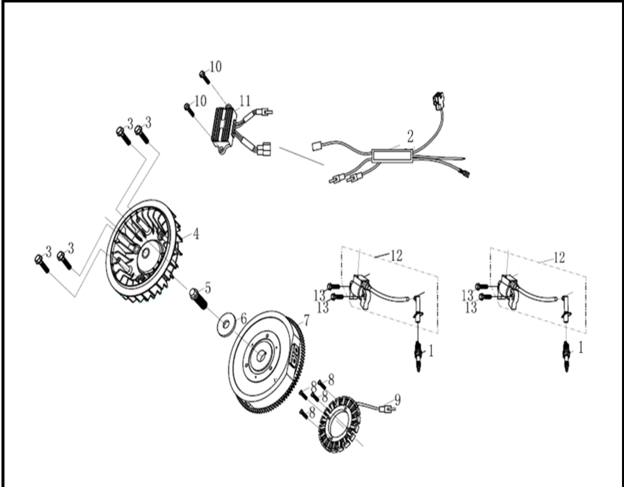
Flywheel/Coil Assy
