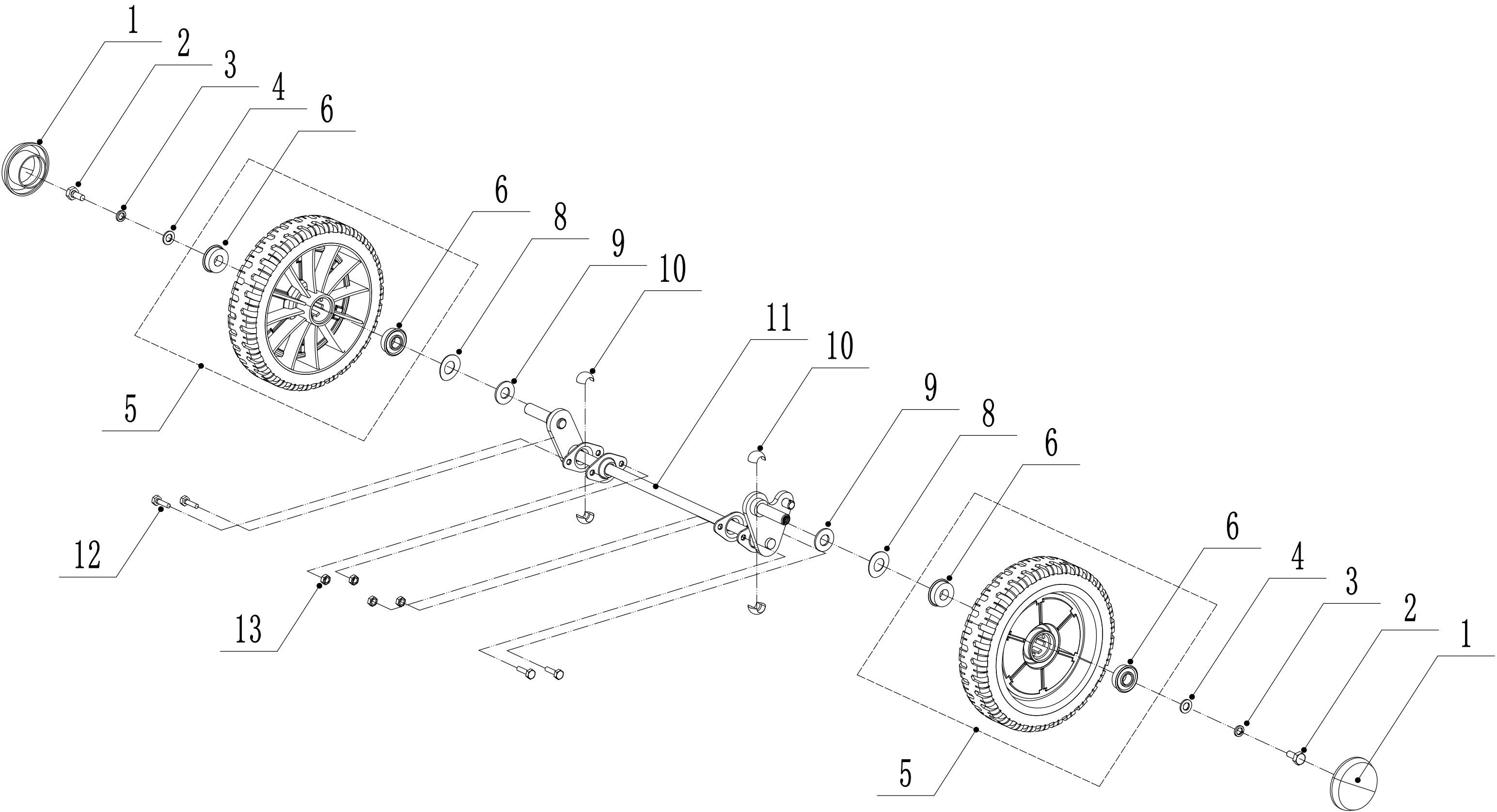
4 Front Axle
