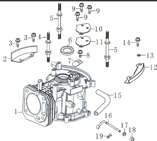
曲轴箱 (CRANK CASE)
